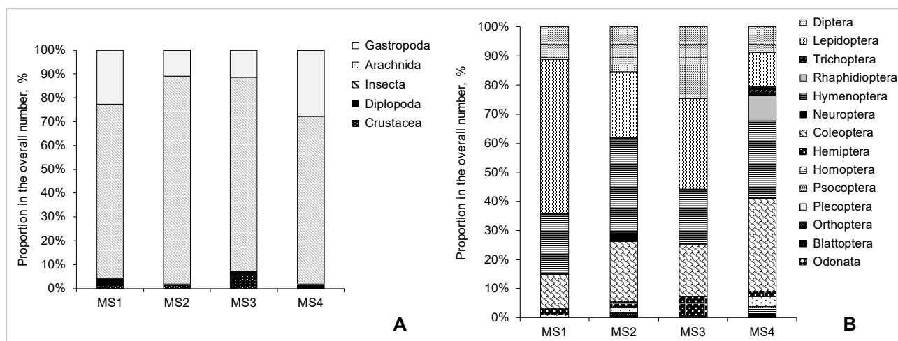
Figure 2. Diversity of trophic links in the collared flycatcher: A – main groups of invertebrates; B – main orders of insects
