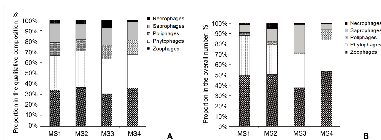
Figure 4. Distribution of trophic groups in the diet of collared flycatcher nestlings across the four study sites: A – proportion in the qualitative composition, B – proportion in the overall number
