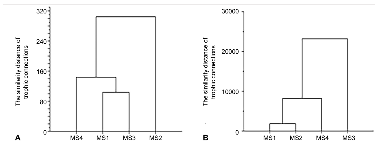
Figure 3. Similarity of trophic links of the collared flycatcher in the studied sites (A – by the qualitative structure of diet; B – by diversity indices)
