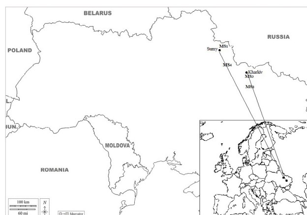
Figure 1. The sites, where the invertebrates from the diet of collared flycatcher nestlings ( Ficedula albicollis ) were collected in transformed forest ecosystems in north-eastern Ukraine: MS1 – Vakalivshchyna, MS2 – NNP Homilshanski Forests, MS3 – the forest park of Kharkiv city, MS4 – NNP Hetmanskyi
