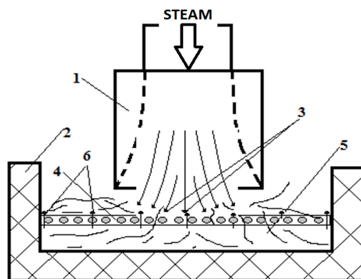
Figure 1. Technological scheme for supplying 100°C wet water steam on oak acorns: 1 – steam diffuser; 2 – thermal insulation box; 3 – steam flow; 4 – grid with oak acorns; 5 – high temperature environment; 6 – temperature sensors
